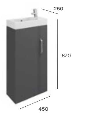
450mm 1 door basin and base unit
